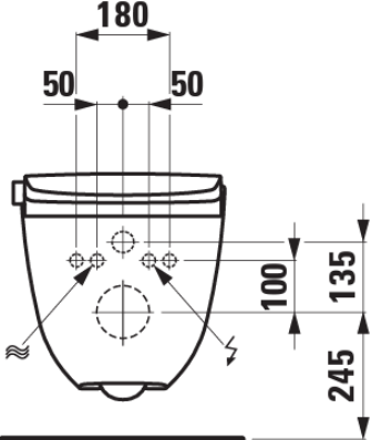
Connection with commercially available installation systems
