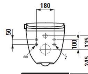
Connection with Laufen installation system LIS CW2
