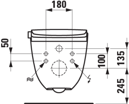
Connection with Laufen installation system LIS CW2
